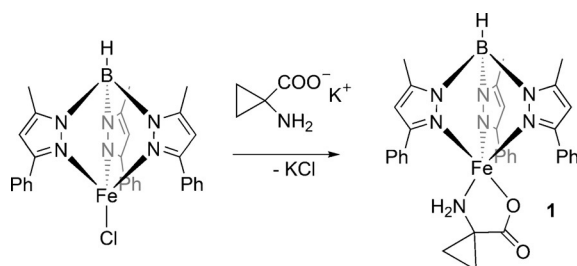
Scheme 2. Synthesis of [Tp^{Me,Ph}FeACC] ( 1 ).
